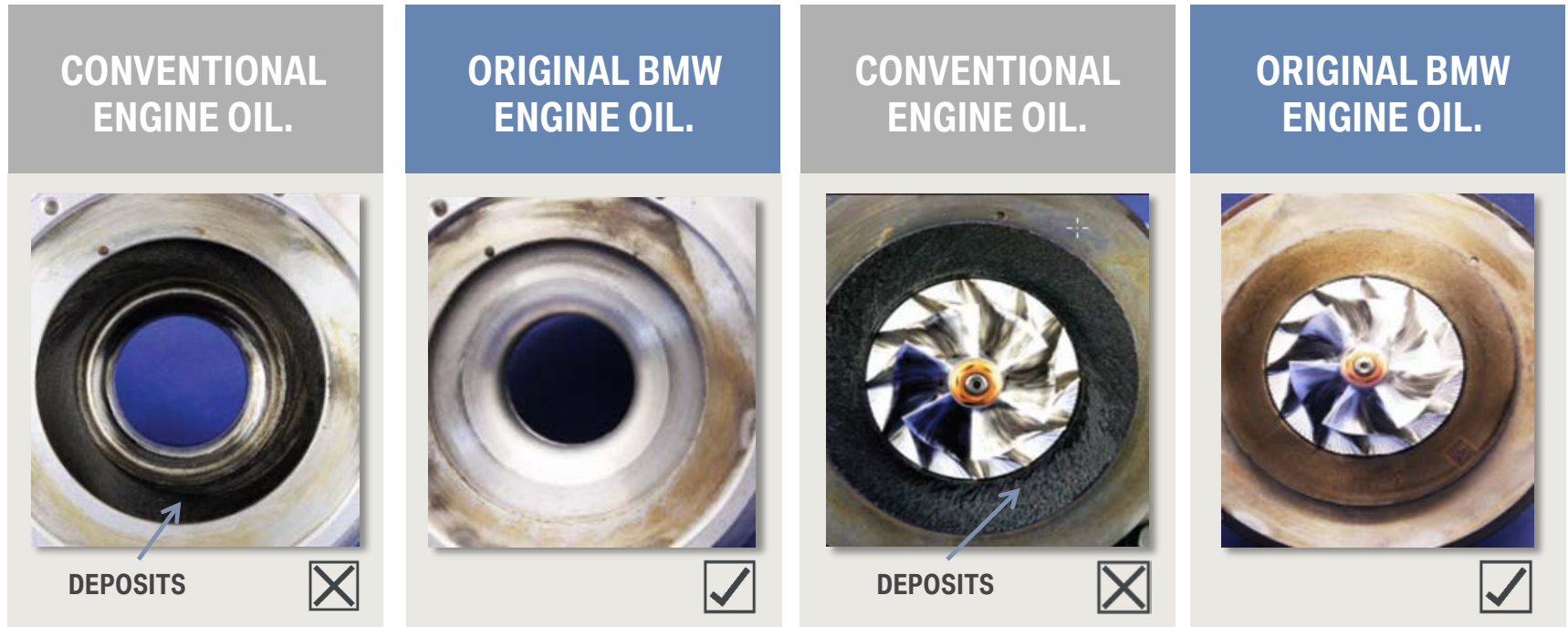
Images show compressor back plate and housing. Tests have been conducted on a turbocharged BMW N47 under high temperature operation.
